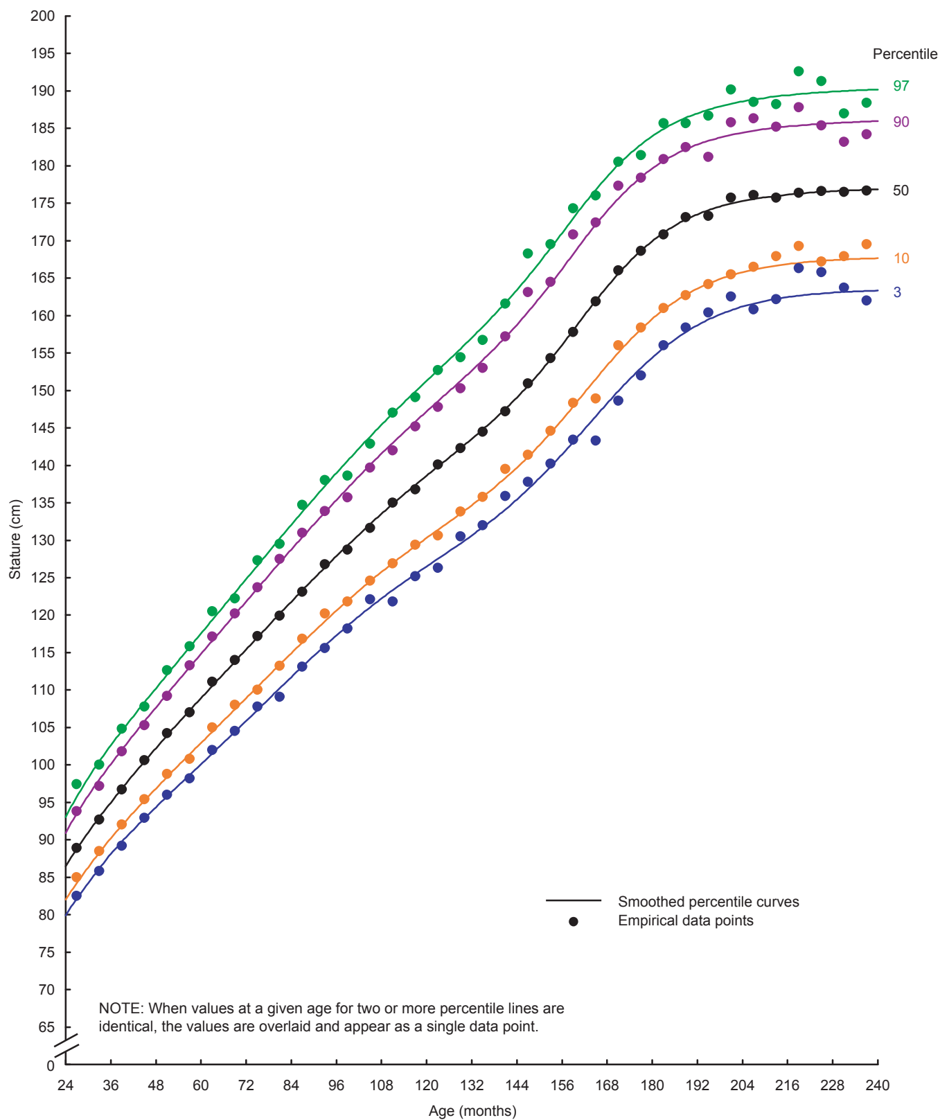
Figure 55. Comparison of smoothed 3rd, 10th, 50th, 90th, 97th percentile curves to empirical data points, 24–237 months: Boys stature-for-age
