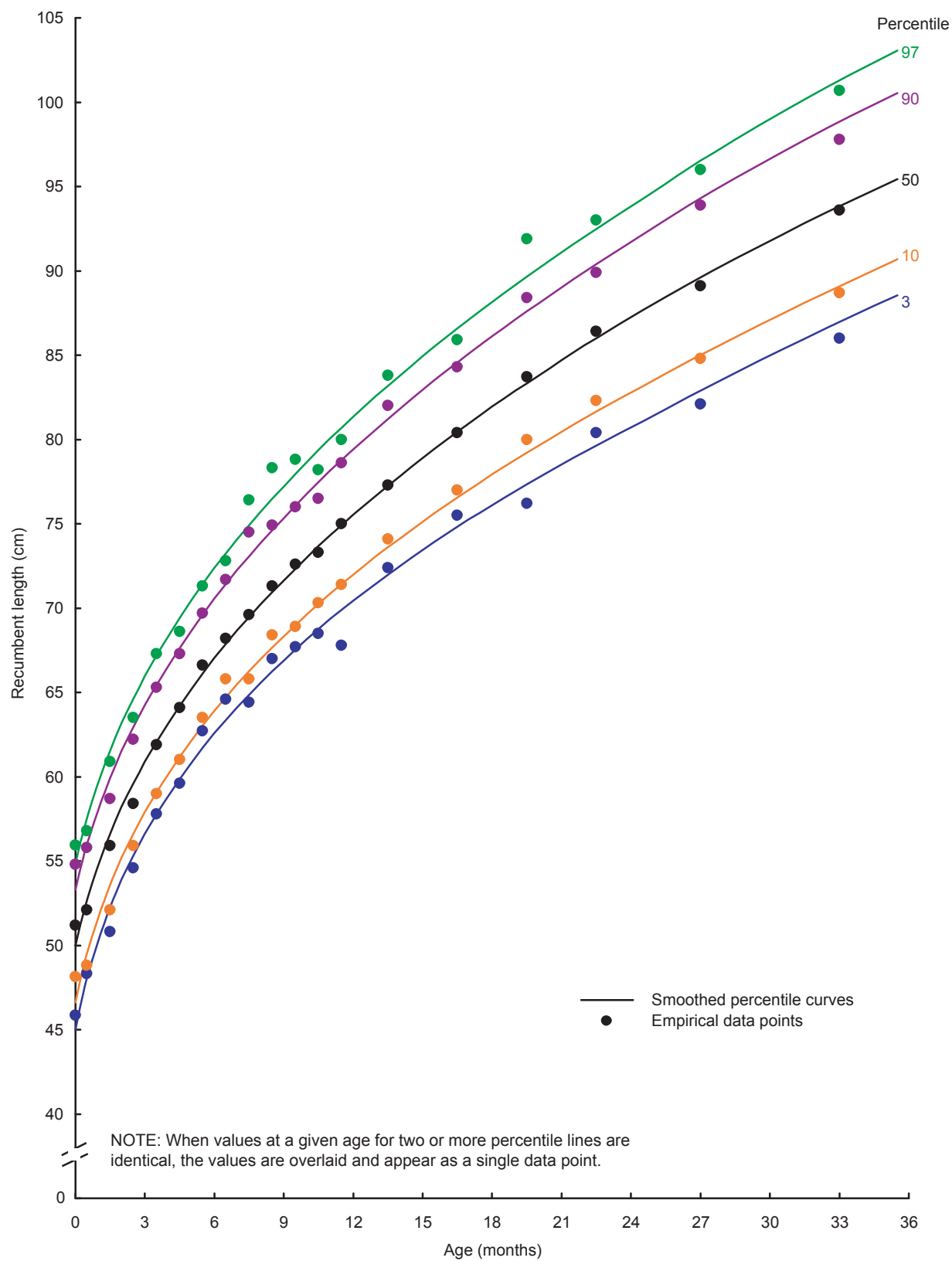
Figure 35. Comparison of smoothed 3rd, 10th, 50th, 90th, 97th percentile curves to empirical data points, birth to 36 months: Boys recumbent length-for-age
