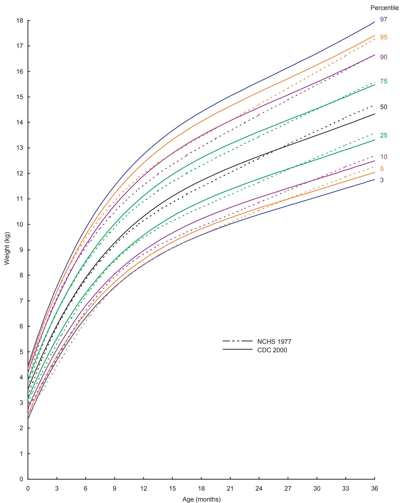
Figure 95. Comparison of CDC 2000 smoothed 3rd, 5th, 10th, 25th, 50th, 75th, 90th, 95th, 97th percentiles with NCHS 1977 smoothed 5th, 10th, 25th, 50th, 75th, 90th, 95th percentile curves, birth to 36 months: Boys weight-for-age
