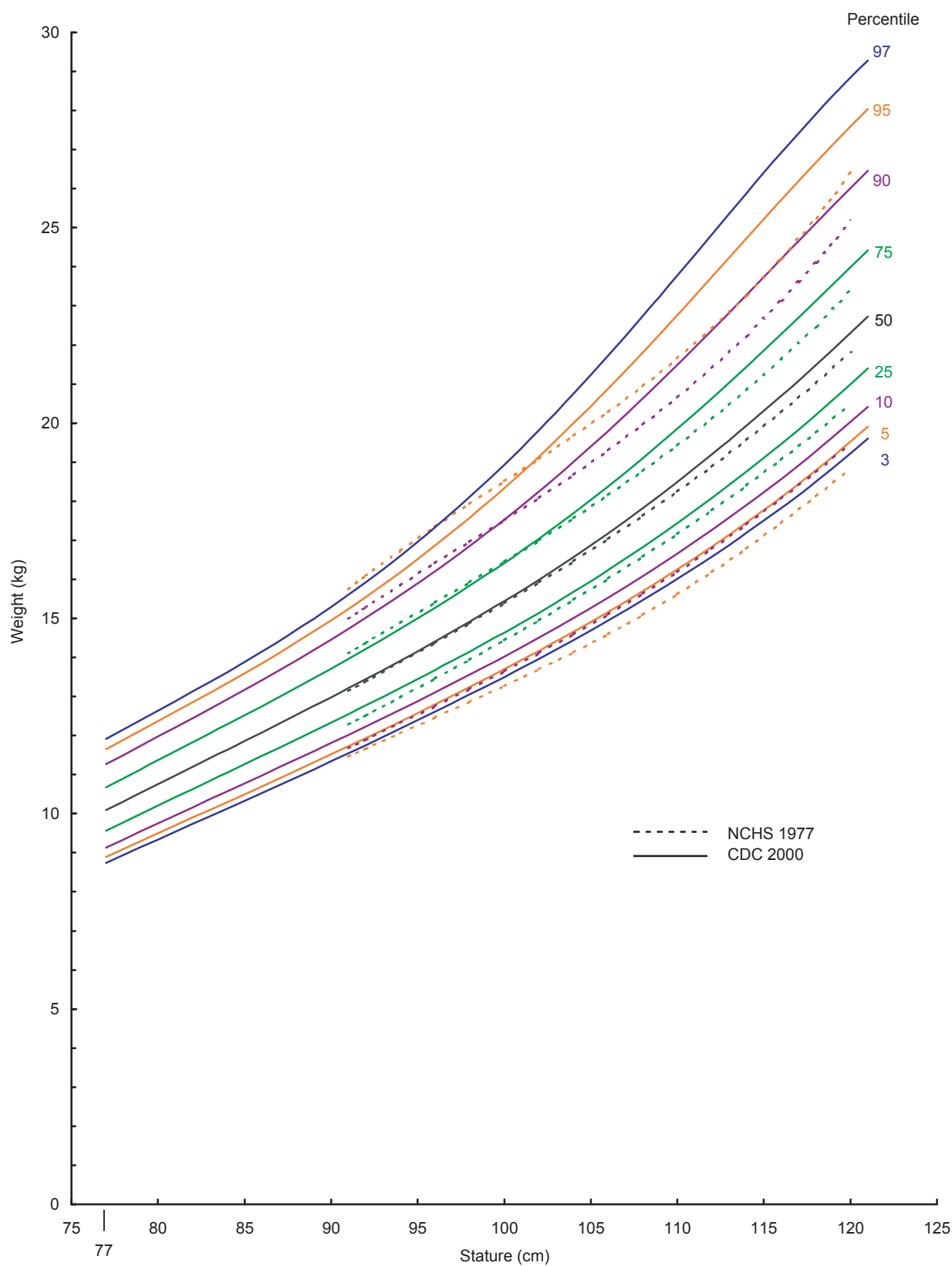
Figure 104. Comparison of CDC 2000 smoothed 3rd, 5th, 10th, 25th, 50th, 75th, 90th, 95th, 97th percentiles with NCHS 1977 smoothed 5th, 10th, 25th, 50th, 75th, 90th, 95th percentile curves, 91–120 cm: Girls weight-for-stature
