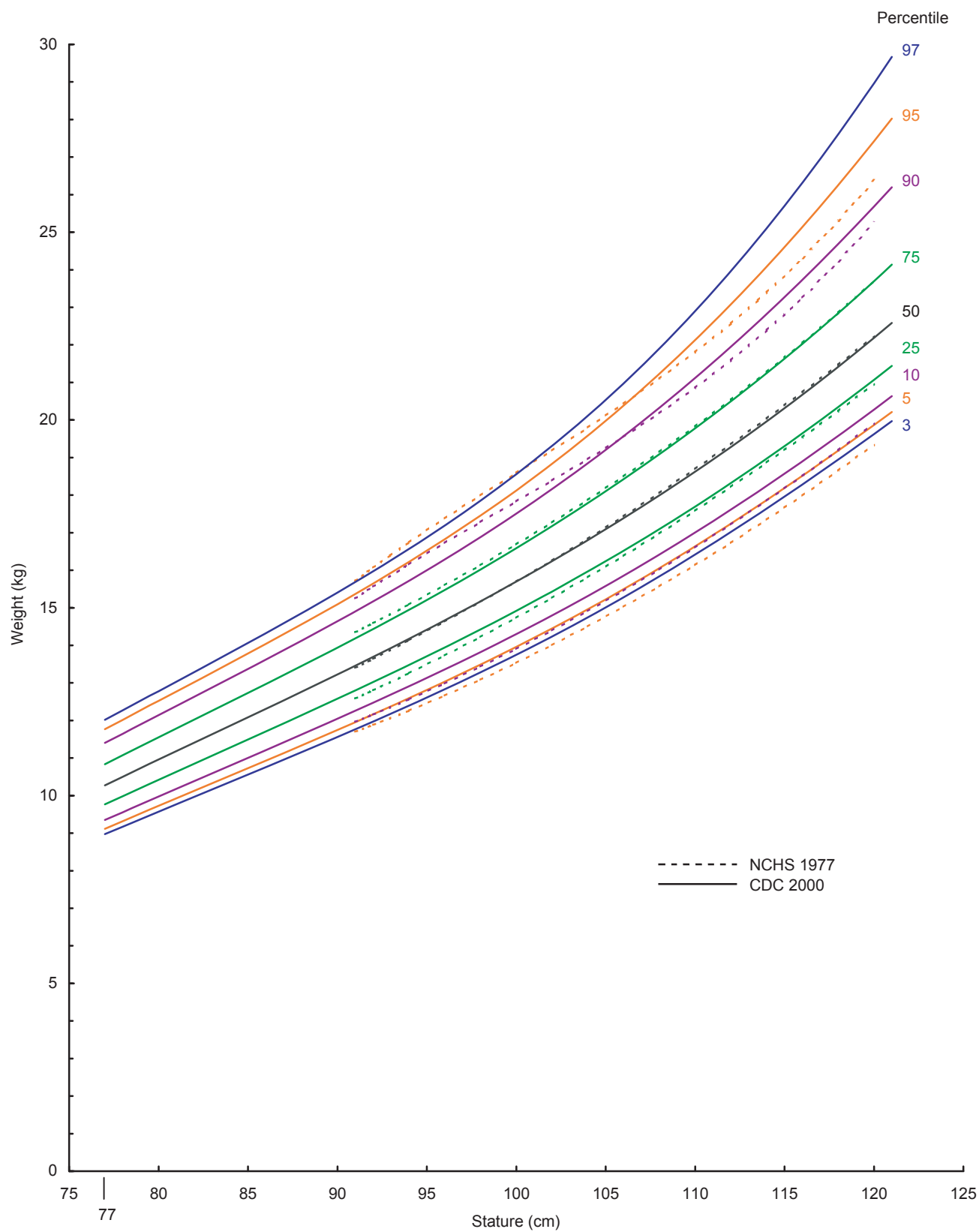
Figure 103. Comparison of CDC 2000 smoothed 3rd, 5th, 10th, 25th, 50th, 75th, 90th, 95th, 97th percentiles with NCHS 1977 smoothed 5th, 10th, 25th, 50th, 75th, 90th, 95th percentile curves, 91–120 cm: Boys weight-for-stature
