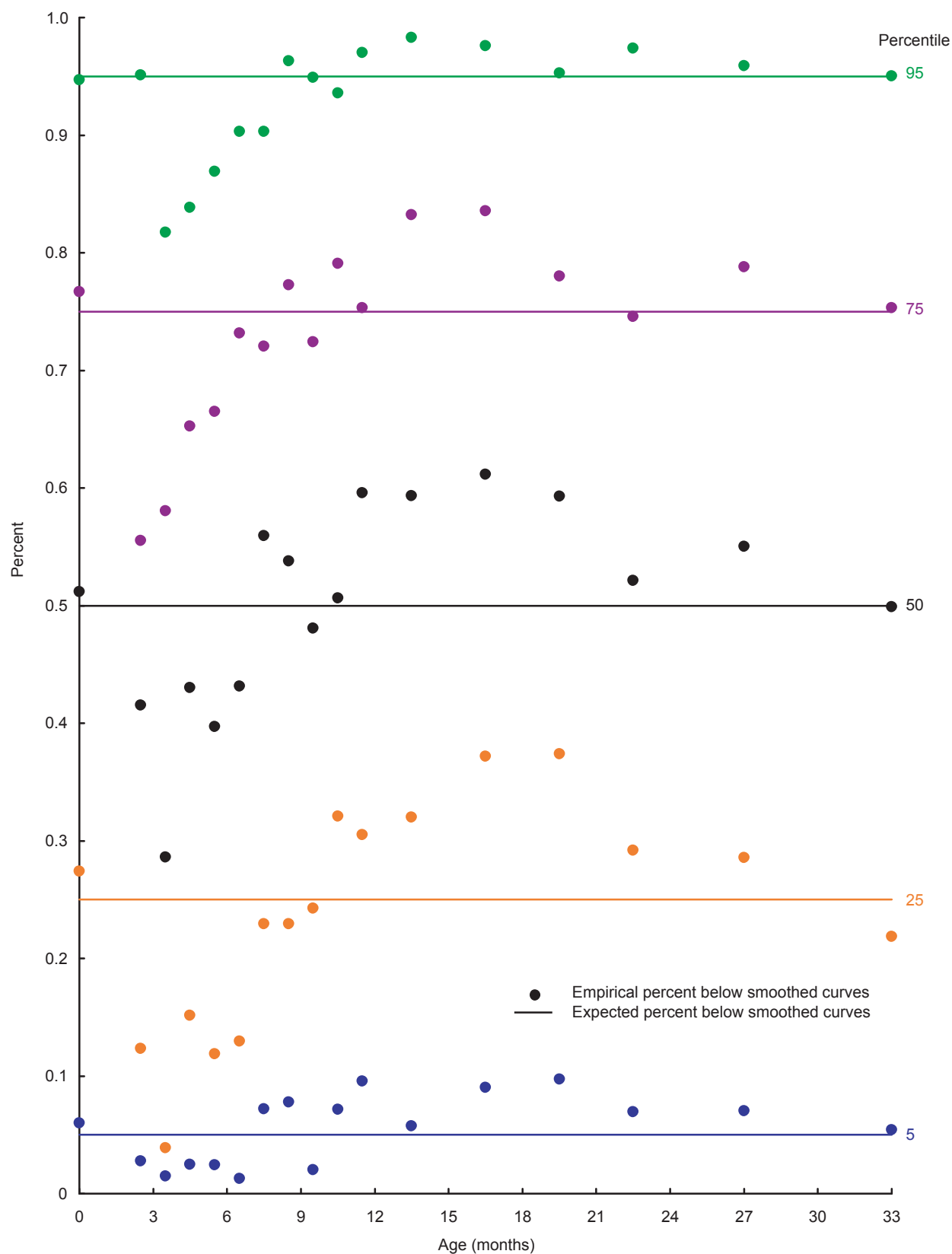
Figure 66. Percent of empirical data below smoothed 5th, 25th, 50th, 75th, 95th percentile curves, birth to 33 months: Girls weight-for-age
