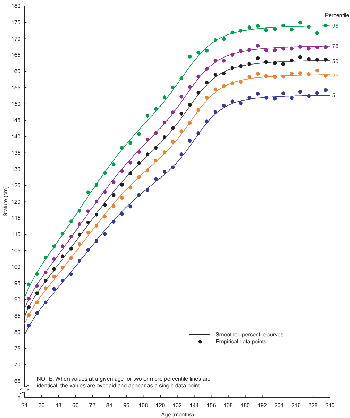
Figure 58. Comparison of smoothed 5th, 25th, 50th, 75th, 95th percentile curves to empirical data points, 24–237 months: Girls stature-for-age
