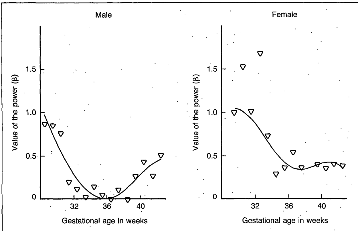
Figure 2. Values of the power ( \beta ) for each gestational age 28–42 weeks, by sex: Sweden, 1977–78
